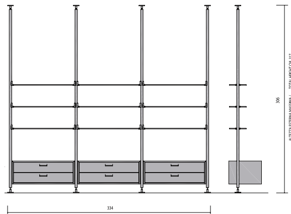
COMP. U50
