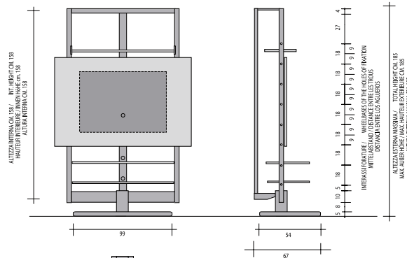
COMP. U41
